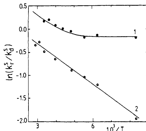
Figure 4. Temperature dependence of the ratio of the phototransfer rate constant ( k_r^s ) of hydrogen (1) or deuterium (2) atom in the excited singlet state of 1-methylanthraquinone to the rate constant of intersystem crossing from this state ( k_d^s ).
