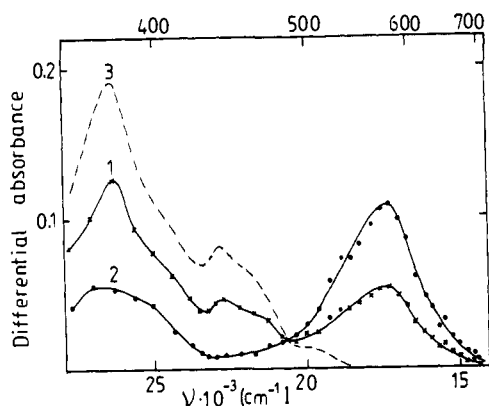
Figure 3. Differential absorption spectrum detected immediately after pulse excitation of 1-methylanthraquinone (1), the absorption spectrum of 9-hydroxy-1,10-anthraquinone-1-methide detected 3.5 \mu s after laser pulse (2), and the absorption spectrum of the triplet intermediate (T) estimated by the formula D(T) = 1.96 D(0) - 0.96 D(3.5 \mu s) , in ethanol at 206 K.
